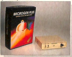
MICROGEN PLUS. Genlock VHS, Superimpose, FADE professionale, Invert Key, porta RGB passante. Banda passante 4,7 Mhz +/- 1Db. MICROGEN PLUS S-VHS. Genlock VHS e S-VHS, Superimpose, FADE professionale, Invert Key, porta RGB passante. Cromo Key. Banda passante 5,7 Mhz +/- 1 Db.
