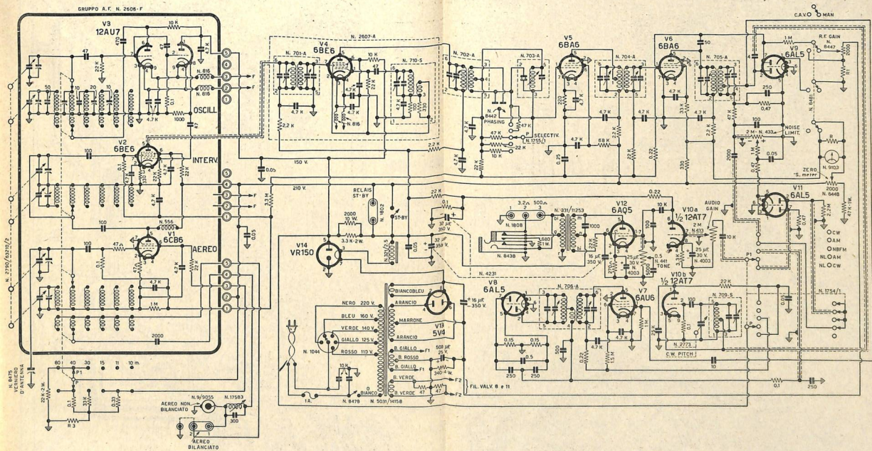
SHORT WAVES RECEIVER MOD. G 207 CR - GELOS0
