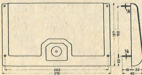
Calibrated Dial Mod. 1640
