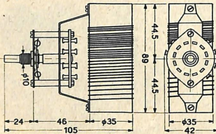
Inductance (switchable) for Final Stage N. 4/110
